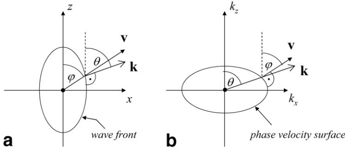
FIG. 1. Schematic 2D illustration of the directional relationship between group velocity \mathbf{v} and wave vector \mathbf{k} in the case of anisotropy. a: If waves emanate from a point source, their group velocity determines the wave front. b: In k -space, the inherent frequencies of a wave field are shown in relation to the phase velocity. Note: \mathbf{k} and \mathbf{v} are only parallel along their principal axes, which is fundamentally different from isotropic elasticity.
